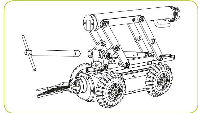
Figure 3.11: Adjusting the large adjustable elevator
