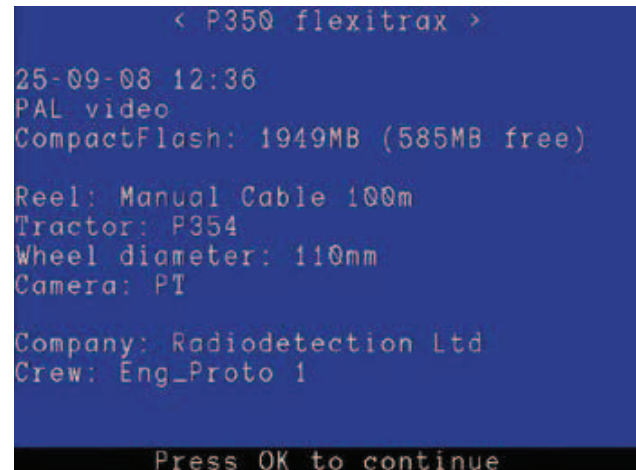
Figure 4.1: Welcome Screen
