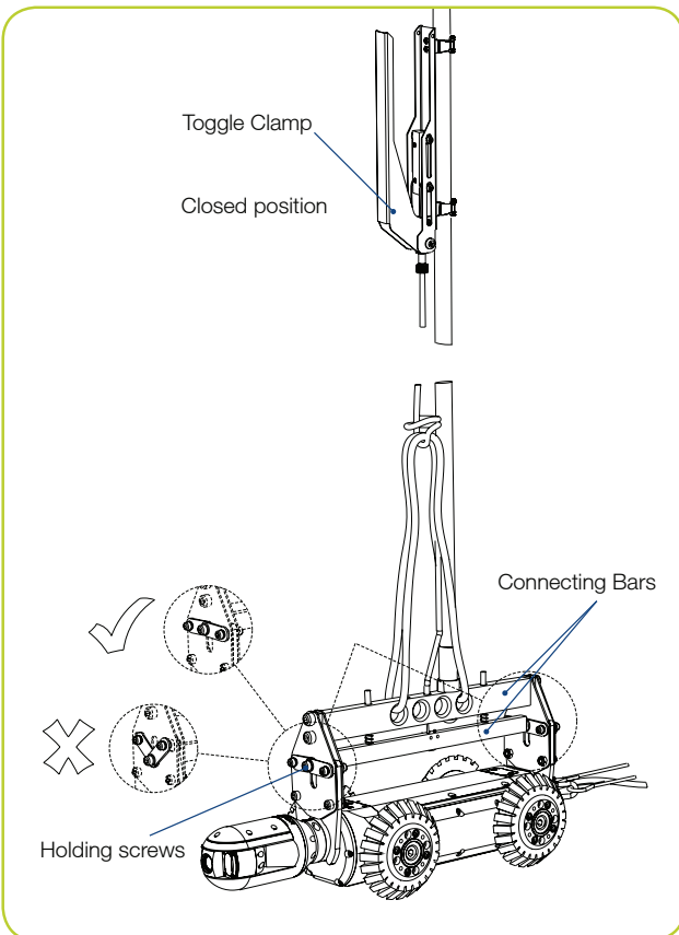
Figure 5.6: Crawler grab in the closed position
