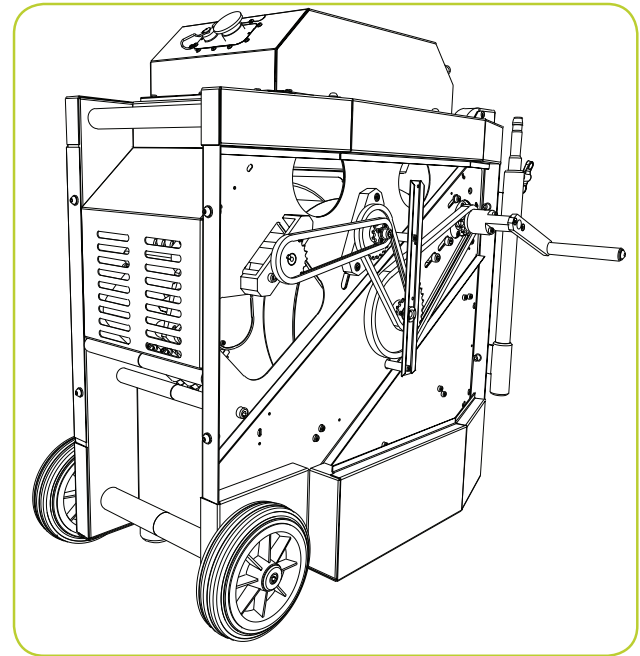
Figure 5.14: Crank handle for powered drum
