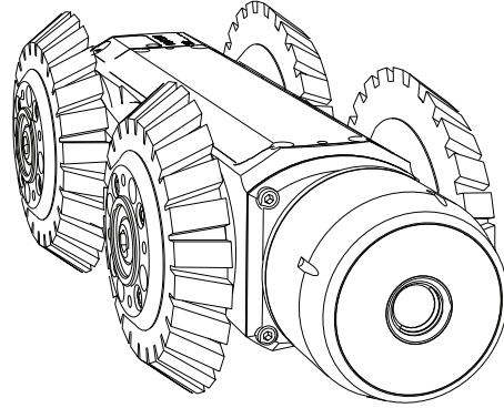
Figure 2.10: P354 crawler with P350-CAM-FW camera installed
