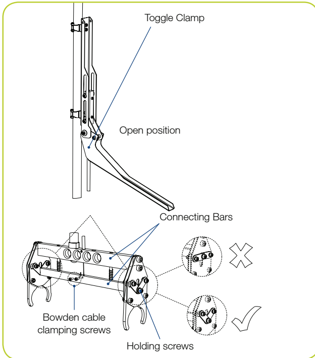
Figure 5.3: Crawler grab setup
