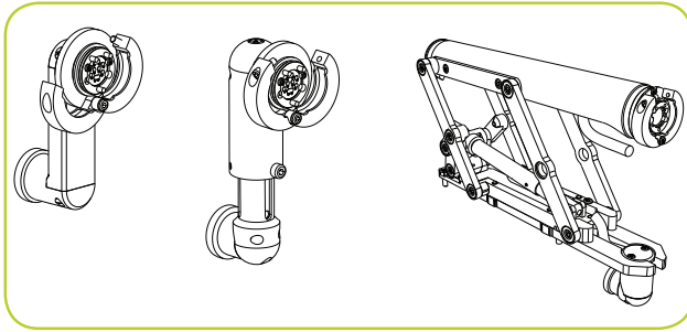
Figure 3.8: P350 camera elevators
