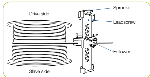
Figure 9.9: Cable layering sprocket and follower
