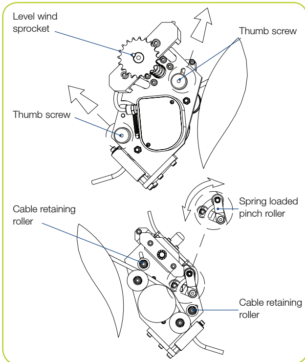
Figure 9.11: Cable drum cassette
