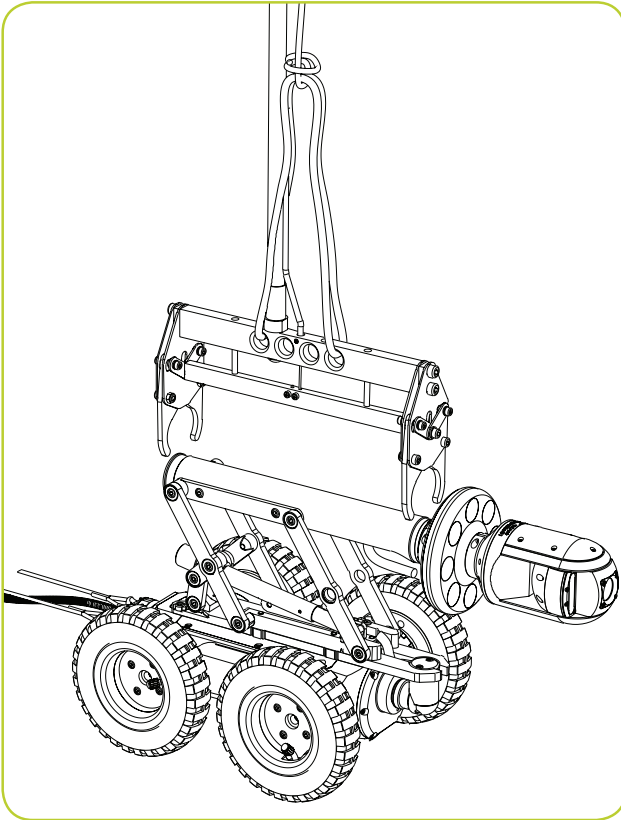
Figure 5.6: Crawler grab in the closed position
