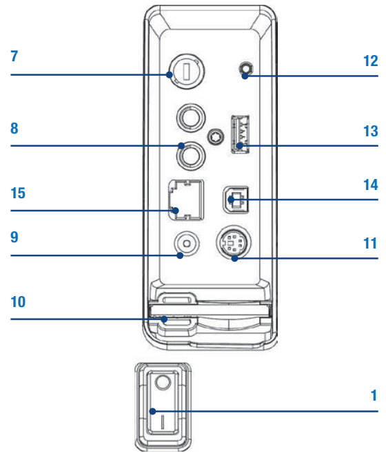
Figure 2.3: Command module I/O panel
