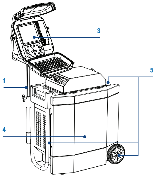
Figure 2.5: Powered drum with command module installed
