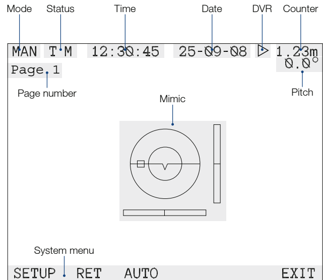
Figure 4.2 System onscreen display (OSD)
