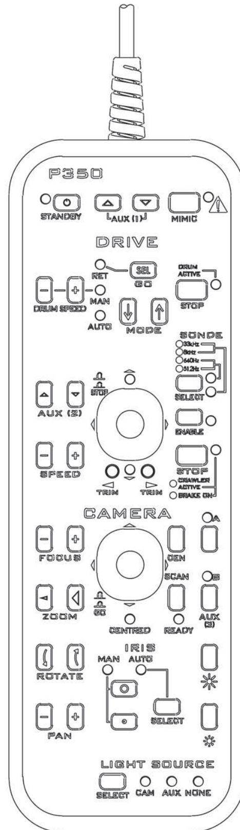
Figure 5.15: Pendant controller
