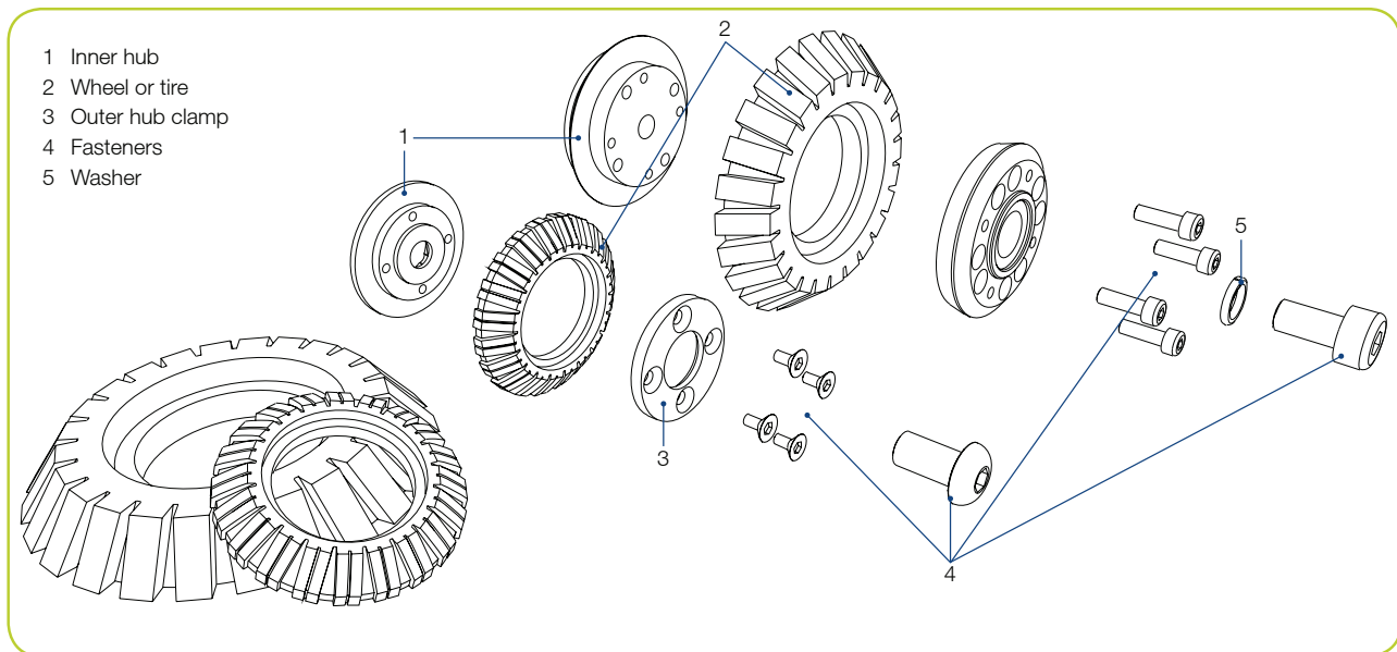
Figure 3.2: Connecting various tires
