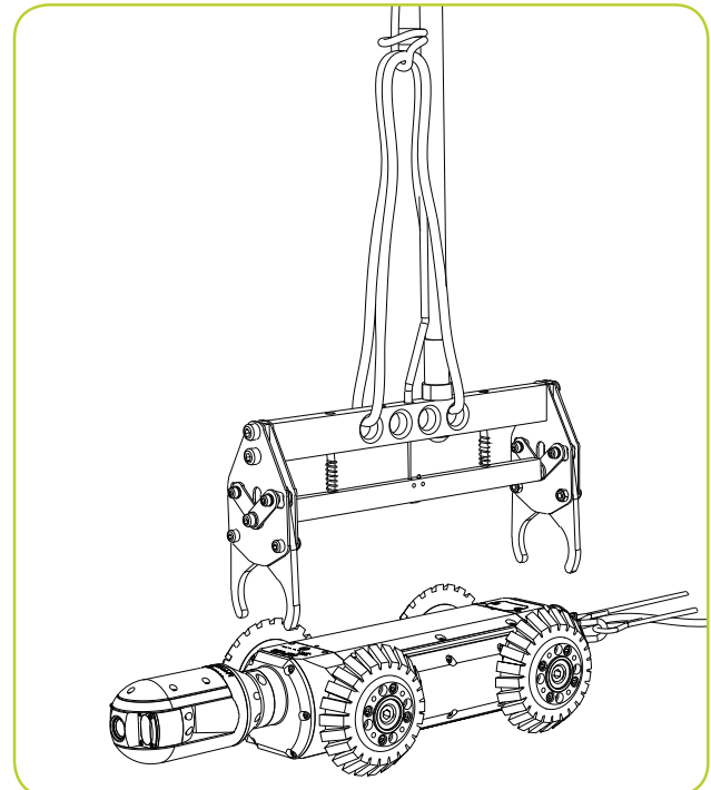
Figure 5.4: Crawler grab and crawler
