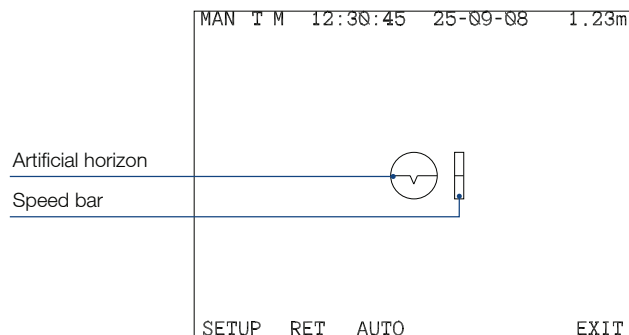
Figure 5.10: Basic mimic
