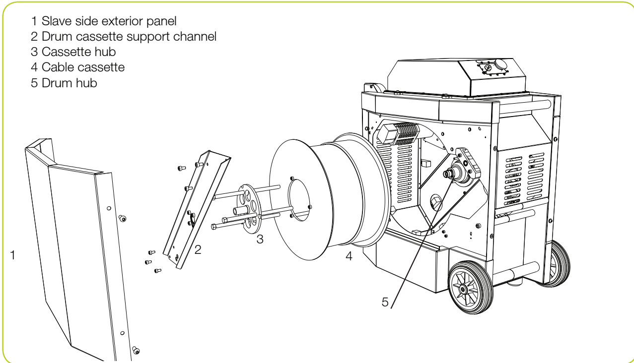
Figure 9.6: Drum cassette replacement (exploded)
