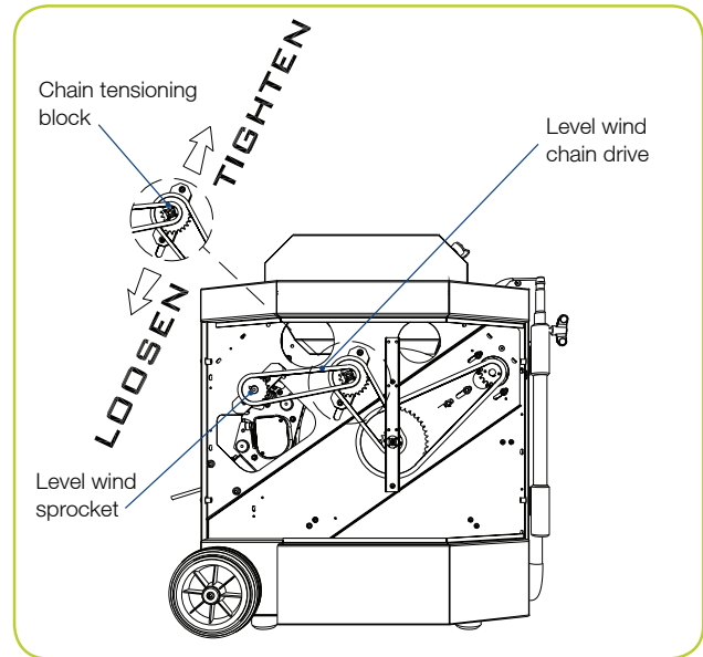
Figure 9.9: Cable layering sprocket and follower
