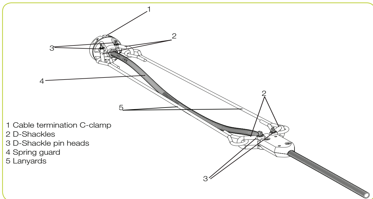
Figure 3.13: Strain relief clamp and spring guard
