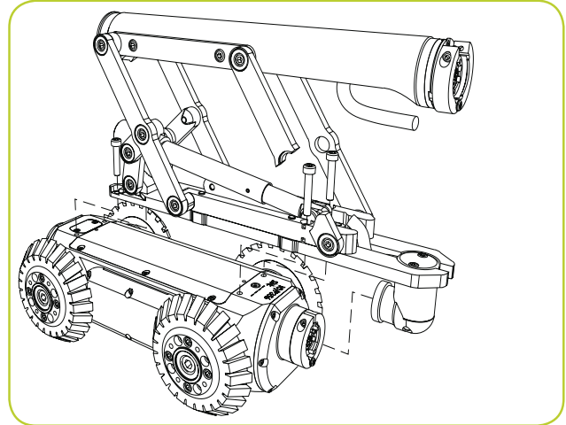
Figure 3.11: Adjusting the large adjustable elevator
