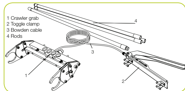
Figure 5.2: Crawler grab kit
