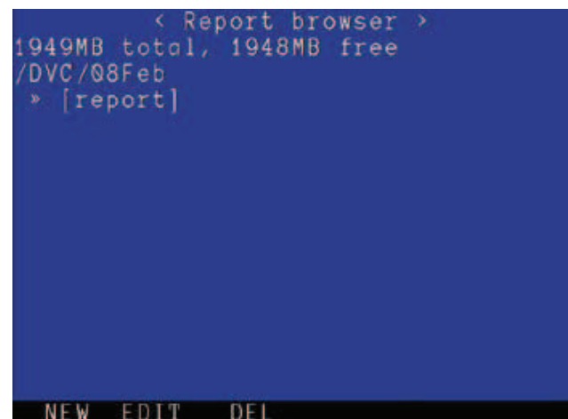
Figure 7.3: Report menu
